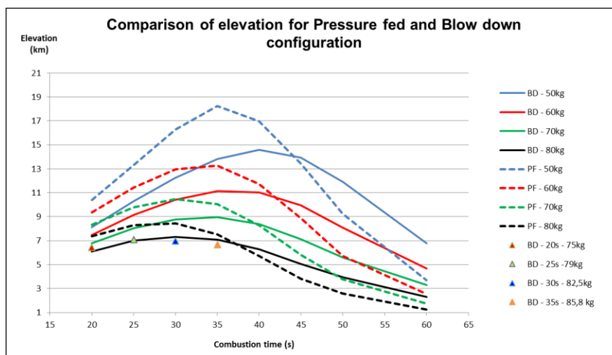
Figure 15 : ASTREOS parametric analysis
