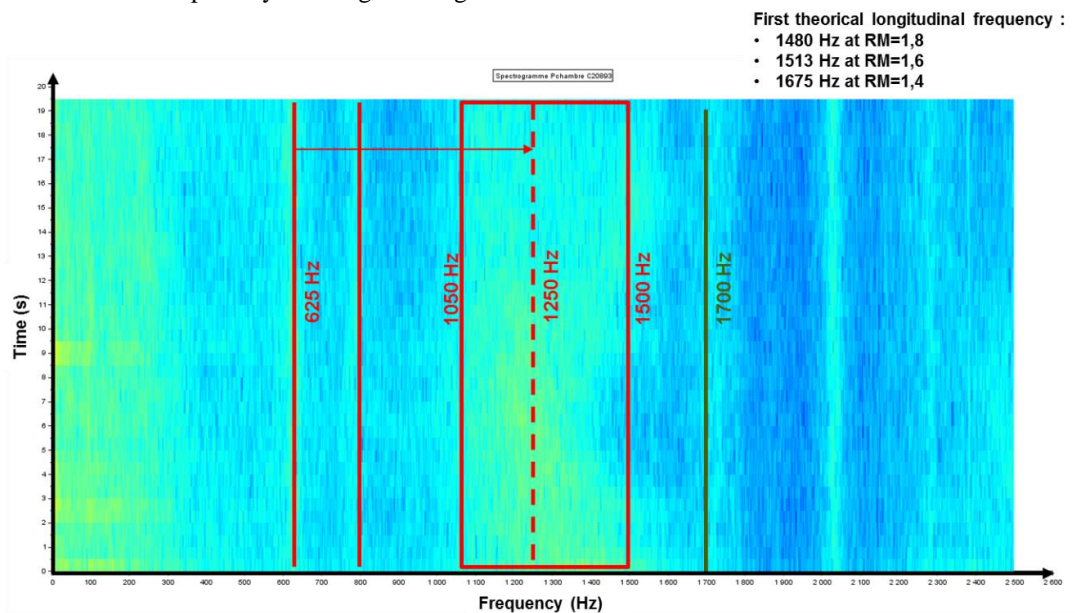
Figure 12 : Frequency analysis
