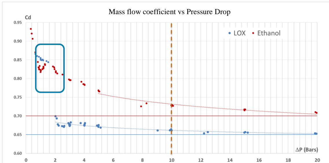
Figure 5 : Cold flow tests results
