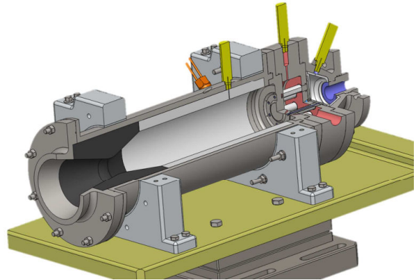
Figure 5: Overview of the first bi-liquid engine for ground fire test.
